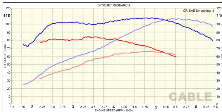
BLUE - 2007 FLHR Muscle 103" Kit with Red Shift 577 and D&D Fatcat vs RED - 2007 FLHR Stock 96"
