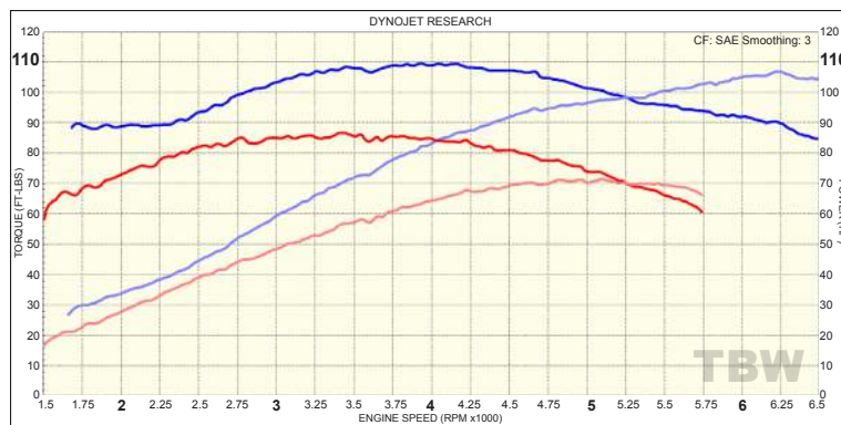
BLUE - 2010 FLHX Muscle 103" Kit with Red Shift 577 vs RED - 2012 FLHR Stock 103"
