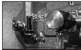
ThunderJet body (nipple down), bowl cent & air bleed jet in place.
