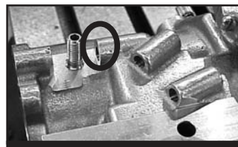
fuel tube hole drilled/tapped, area relieved for T-Jet, fuel tube installed. Circle shows where vent passage should be plugged
